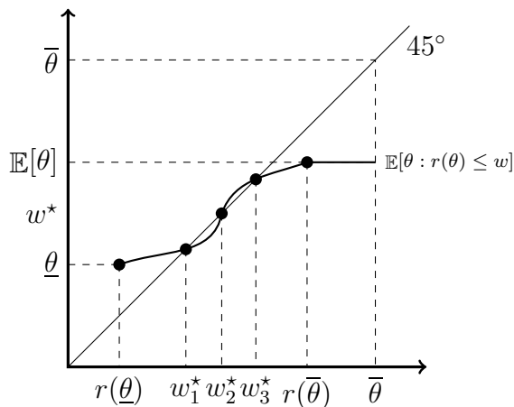
Figure 5: Multiple Equilibria
